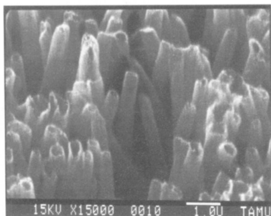
Figure 2. (A, top) Transmission electron micrograph of a microtomed section of an alumina template membrane showing ca. 70-nm-diameter Au nanofibrils within the pores. (B, bottom) Scanning electron micrograph of an array of template-synthesized poly( N -methylpyrrole) tubules. The tubules protrude from an electrode surface.
